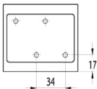
MOUNTING PLATE DETAIL
