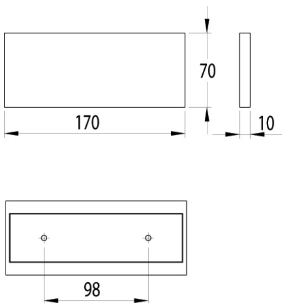
MOUNTING PLATE DETAIL
