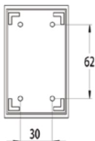
MOUNTING PLATE DETAIL
